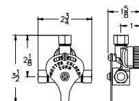
P6900-MT Mixing Tee
